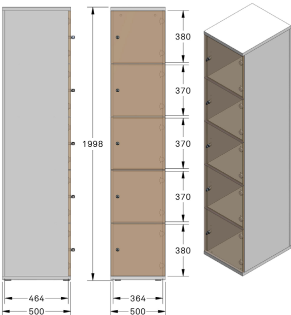
SML5H-4 COMPARTMENT INTERNAL SIZES 364 W x 370/380 H x 464 D
