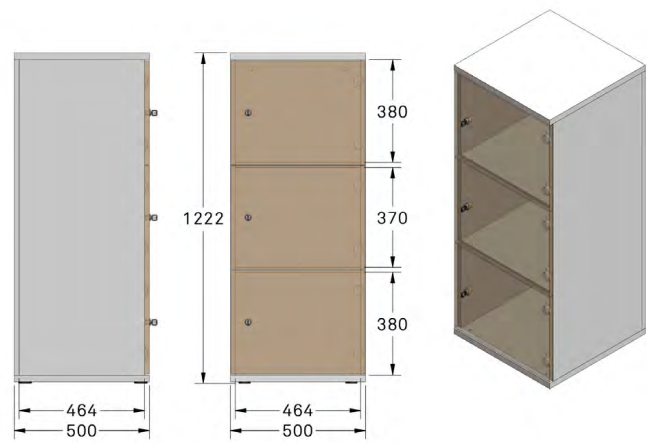
SML3H-5 COMPARTMENT INTERNAL SIZES 464 W x 370/380 H x 464 D
