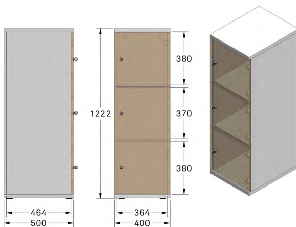
SML3H-4 COMPARTMENT INTERNAL SIZES 364 W x 370/380 H x 464 D
