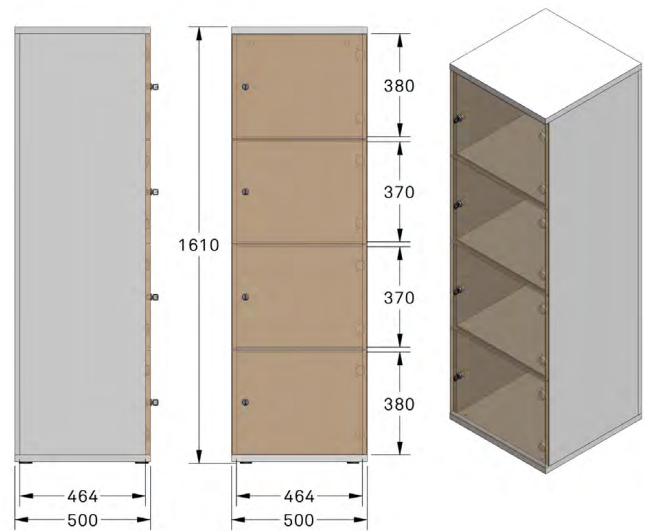
SML4H-5 COMPARTMENT INTERNAL SIZES 464 W x 370/380 H x 464 D
