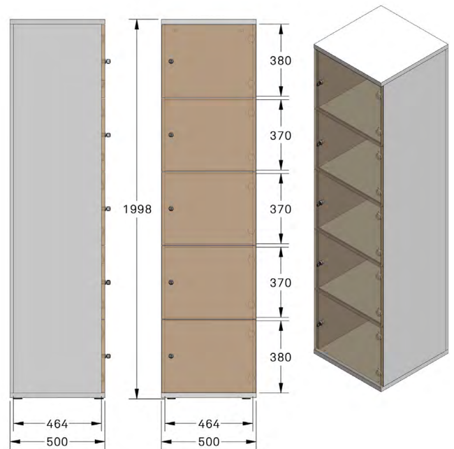
SML5H-5 COMPARTMENT INTERNAL SIZES 464 W x 370/380 H x 464 D
