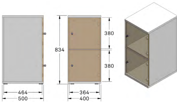
SML2H-4 COMPARTMENT INTERNAL SIZES 364 W x 380 H x 464 D
