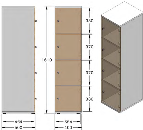
SML4H-4 COMPARTMENT INTERNAL SIZES 364 W x 370/380 H x 464 D
