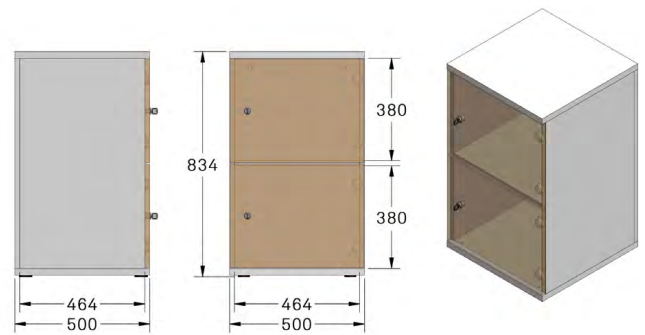
SML2H-5 COMPARTMENT INTERNAL SIZES 464 W x 380 H x 464 D
